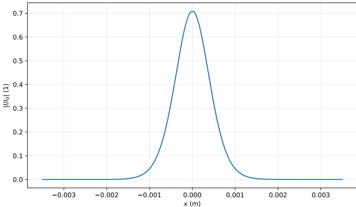
Intensity profile I(x, y = 0, z = 2.070m)/I_0 , P_{in}=0.4P_{cr} , artificial time
